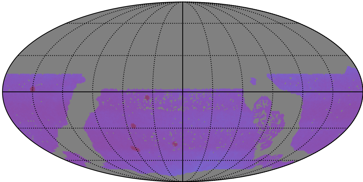
baseline_v3.2_10yrs WFD: Proper Motion Uncert @ 20.5
