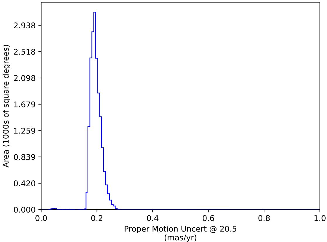
baseline_v3.2_10yrs WFD: Proper Motion Uncert @ 20.5
