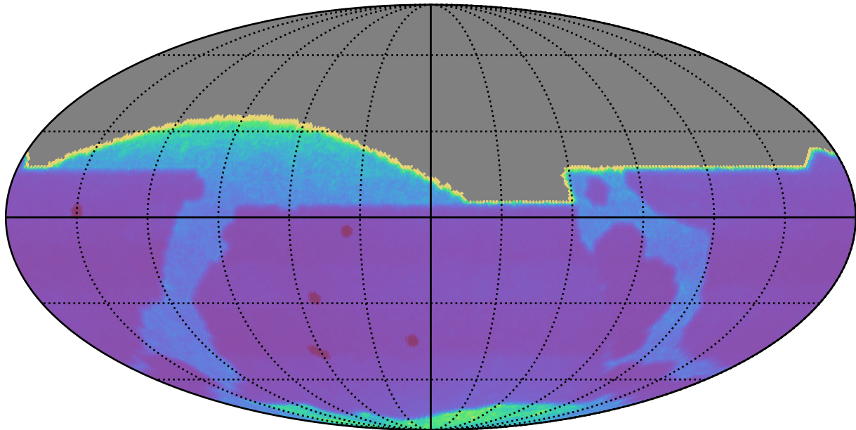
baseline_v3.2_10yrs All sky: Proper Motion Uncert @ 20.5
