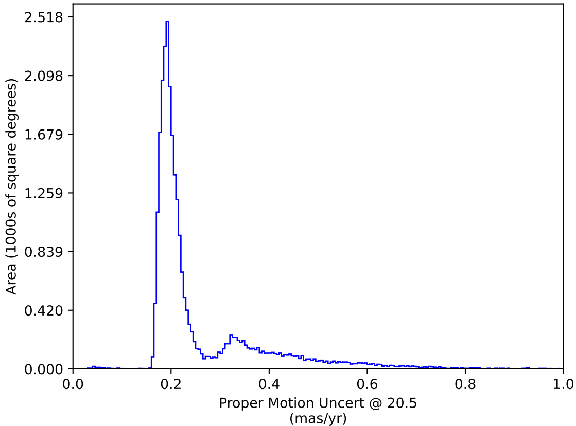
baseline_v3.2_10yrs All sky: Proper Motion Uncert @ 20.5
