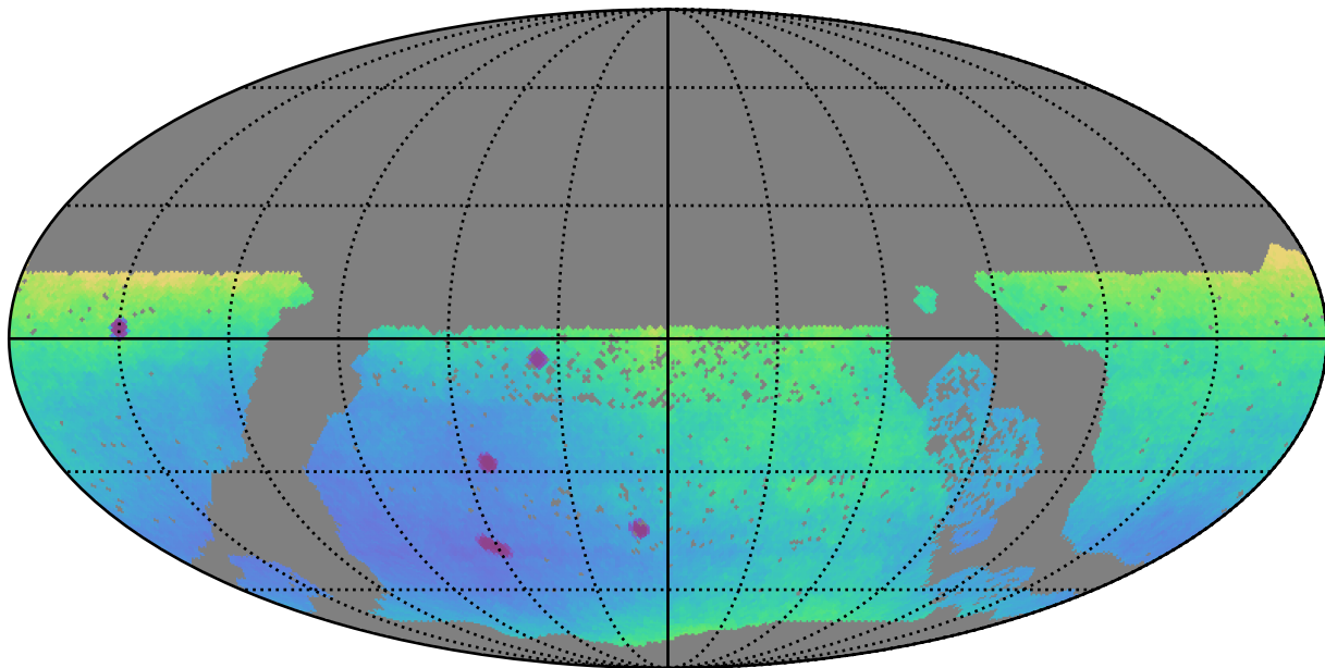
baseline_v3.2_10yrs WFD: Parallax Uncert @ 24.0
