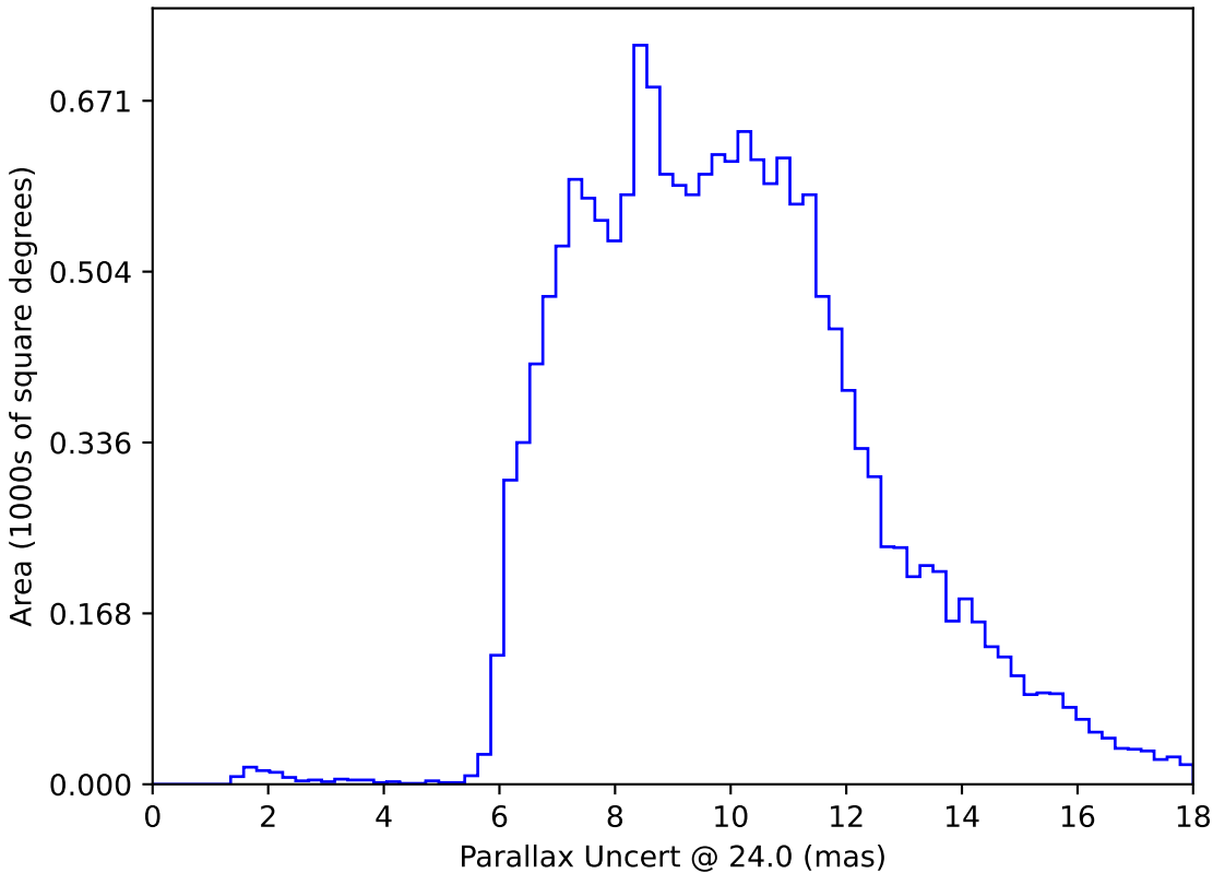
baseline_v3.2_10yrs WFD: Parallax Uncert @ 24.0
