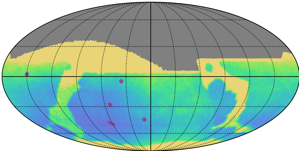
baseline_v3.2_10yrs All sky: Parallax Uncert @ 24.0
