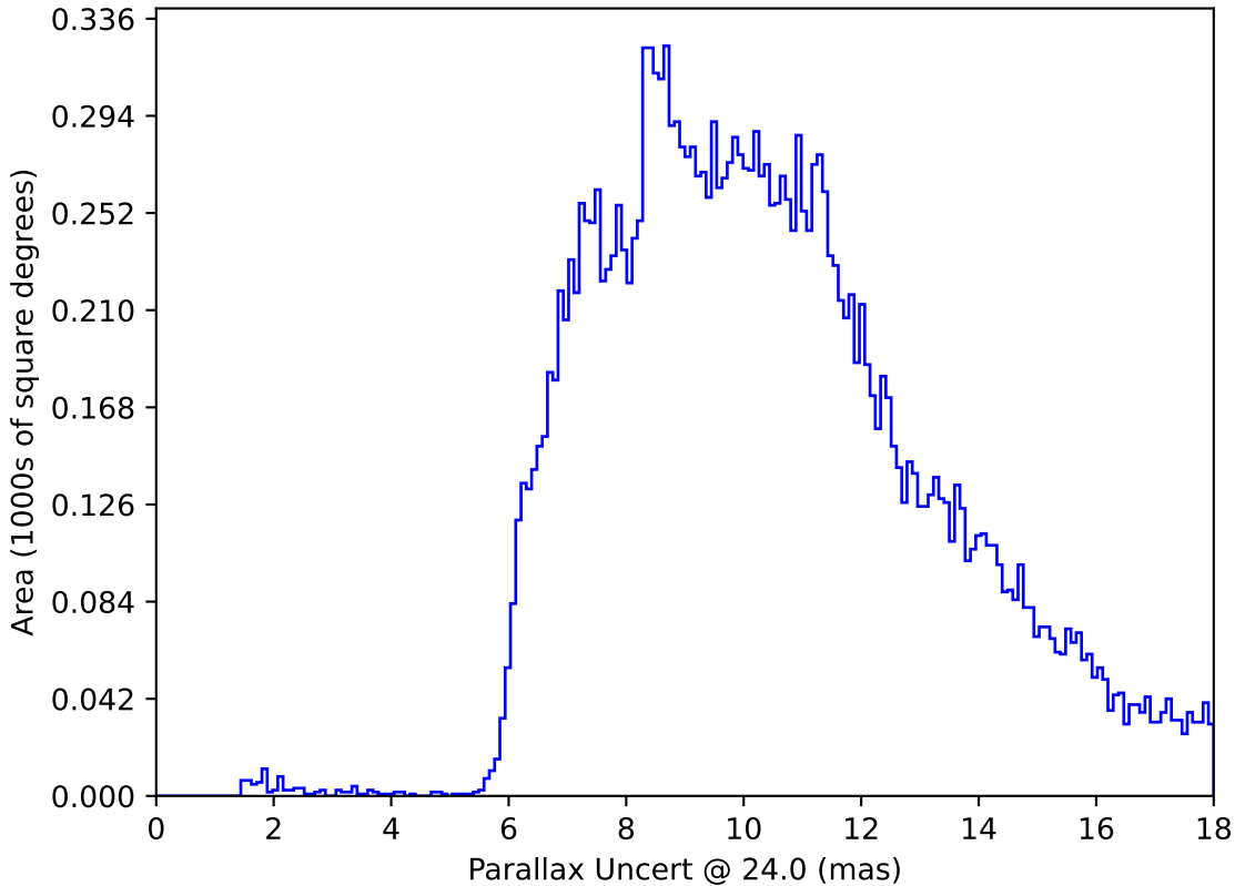
baseline_v3.2_10yrs All sky: Parallax Uncert @ 24.0
