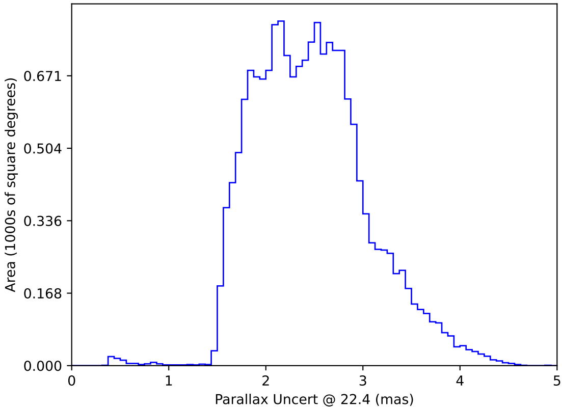
baseline_v3.2_10yrs WFD: Parallax Uncert @ 22.4
