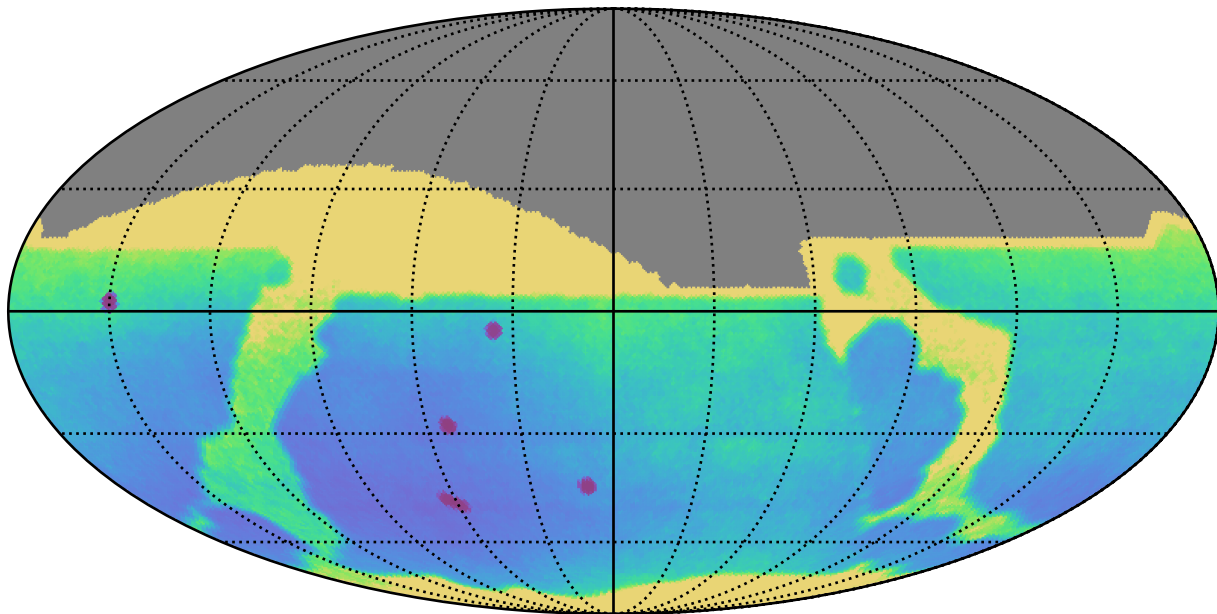
baseline_v3.2_10yrs All sky: Parallax Uncert @ 22.4
