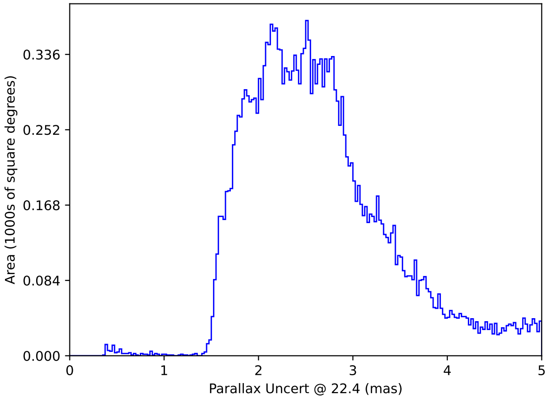
baseline_v3.2_10yrs All sky: Parallax Uncert @ 22.4
