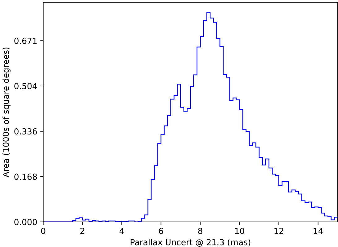
baseline_v3.2_10yrs WFD y band only: Parallax Uncert @ 21.3
