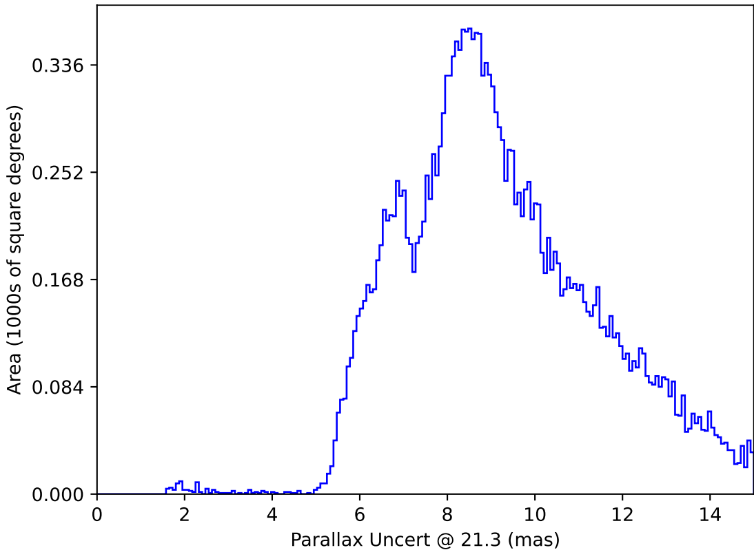
baseline_v3.2_10yrs All sky y band only: Parallax Uncert @ 21.3
