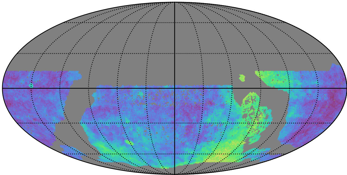
baseline_v3.2_10yrs WFD: Parallax Coverage @ 24.0
