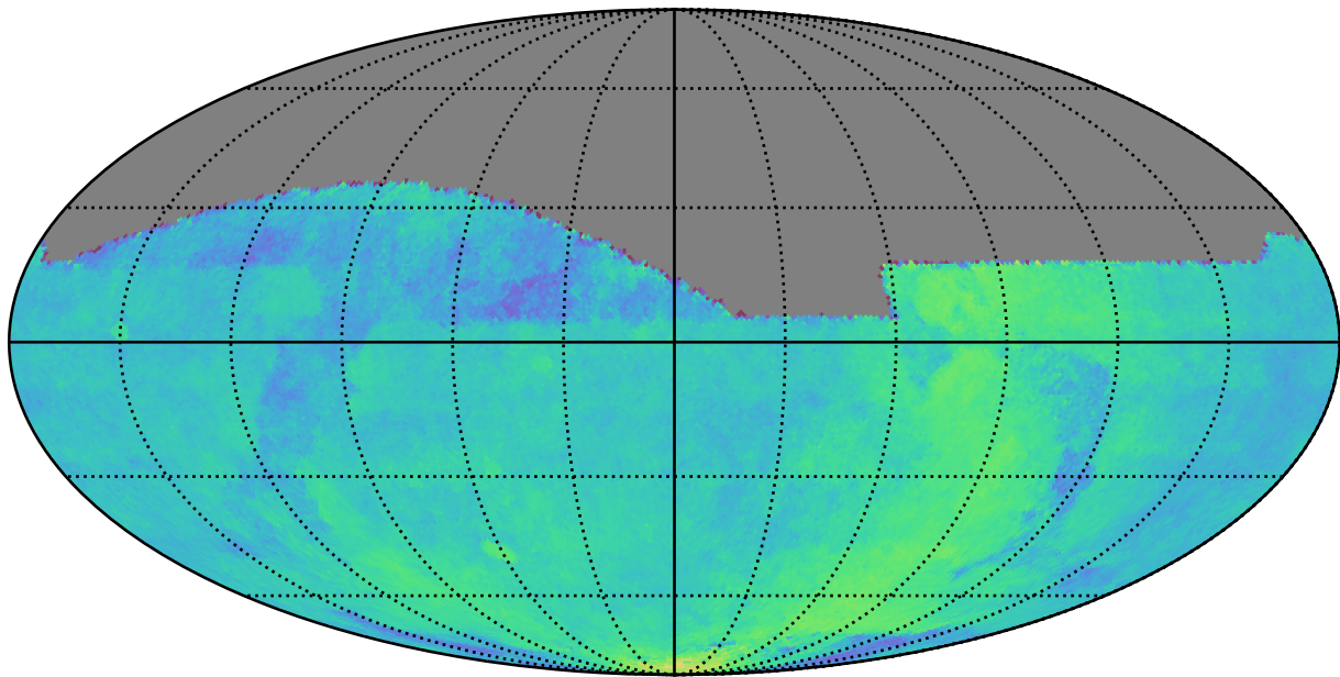
baseline_v3.2_10yrs All sky: Parallax Coverage @ 24.0
