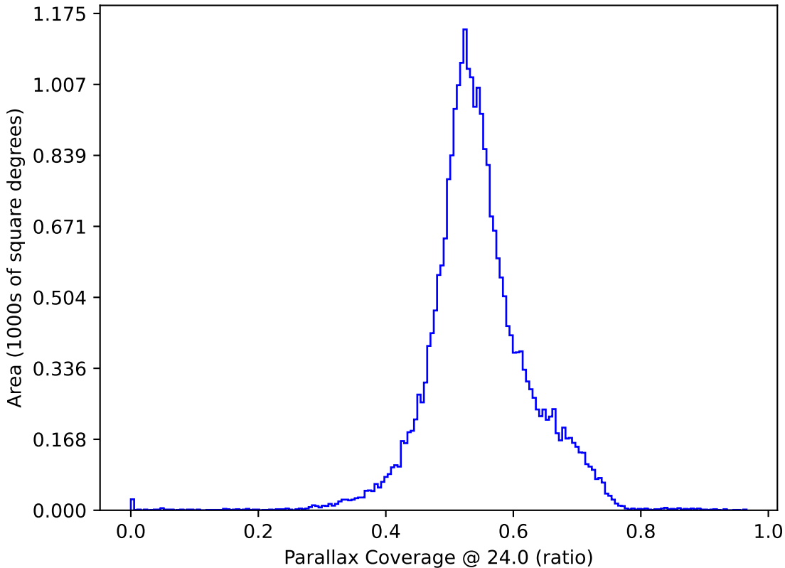
baseline_v3.2_10yrs All sky: Parallax Coverage @ 24.0
