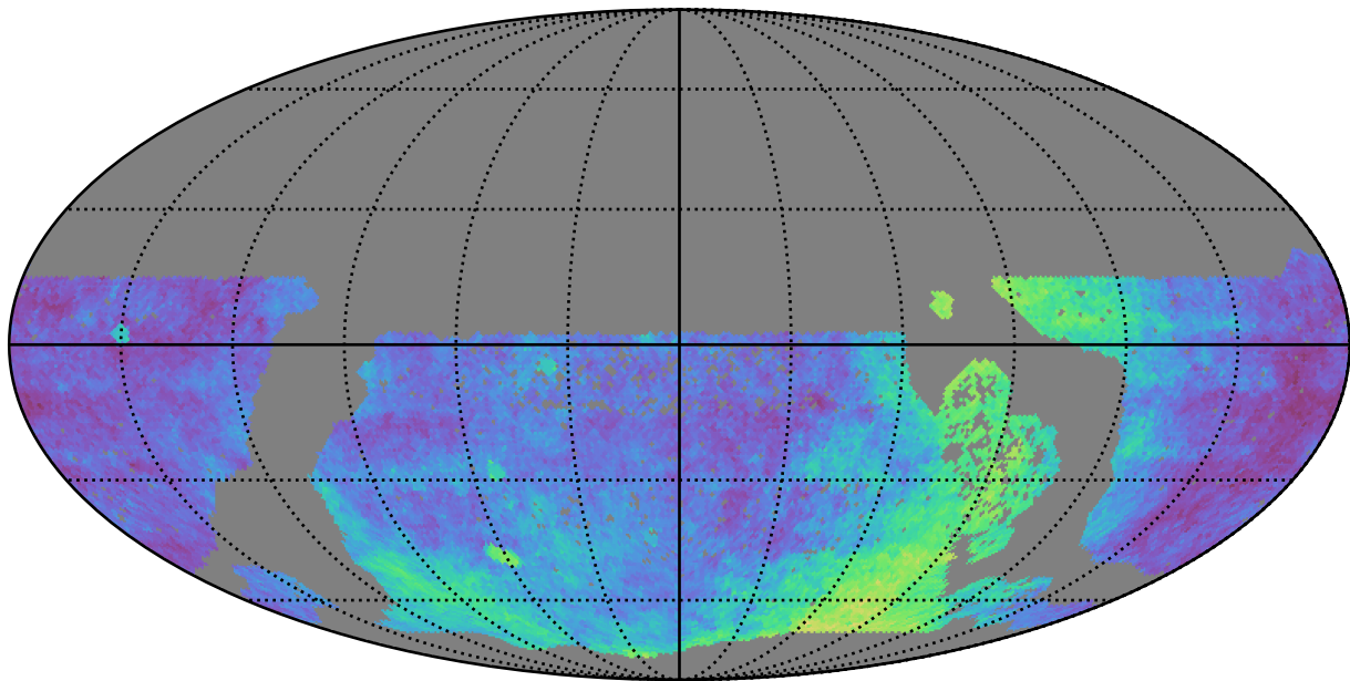
baseline_v3.2_10yrs WFD: Parallax Coverage @ 22.4
