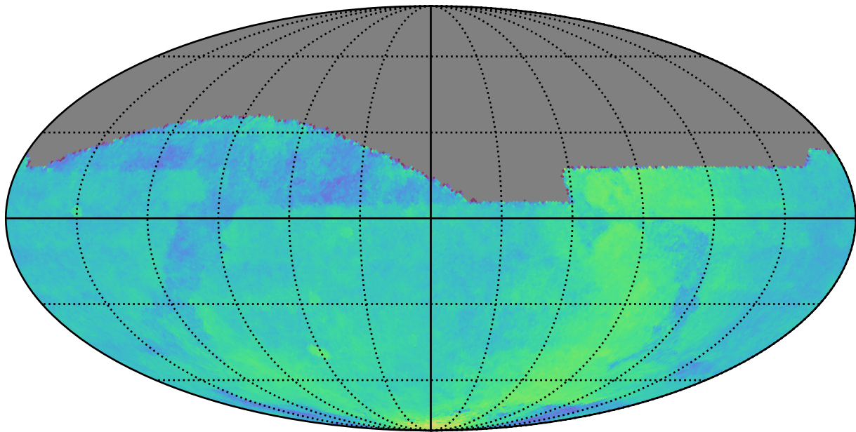
baseline_v3.2_10yrs All sky: Parallax Coverage @ 22.4
