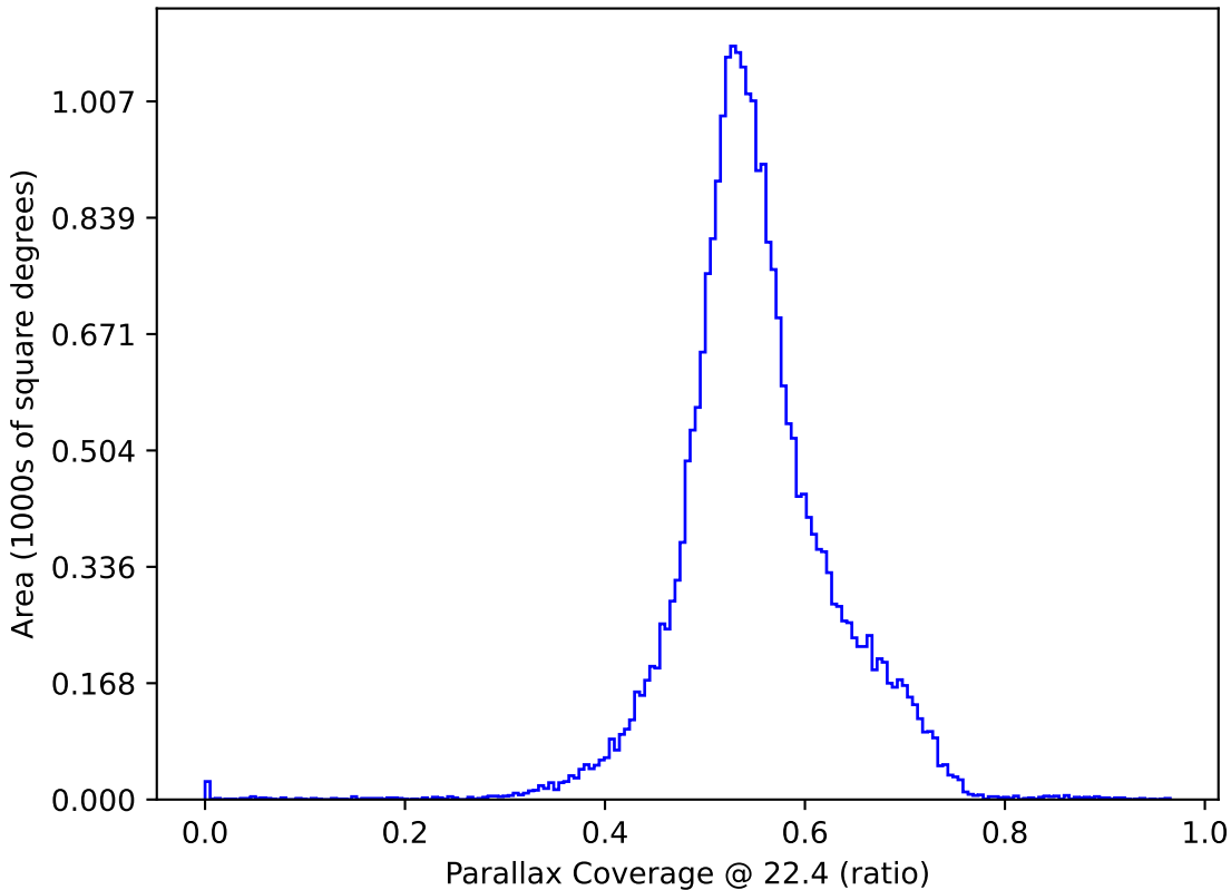
baseline_v3.2_10yrs All sky: Parallax Coverage @ 22.4
