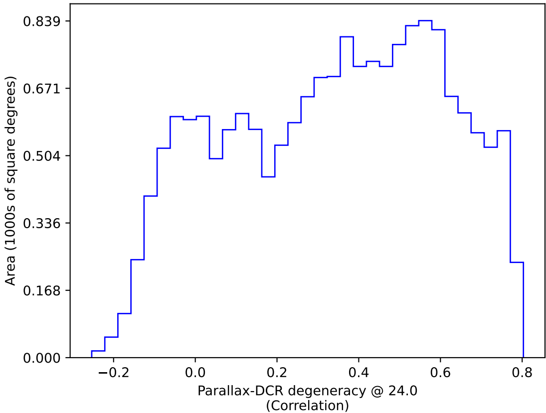
baseline_v3.2_10yrs WFD: Parallax-DCR degeneracy @ 24.0
