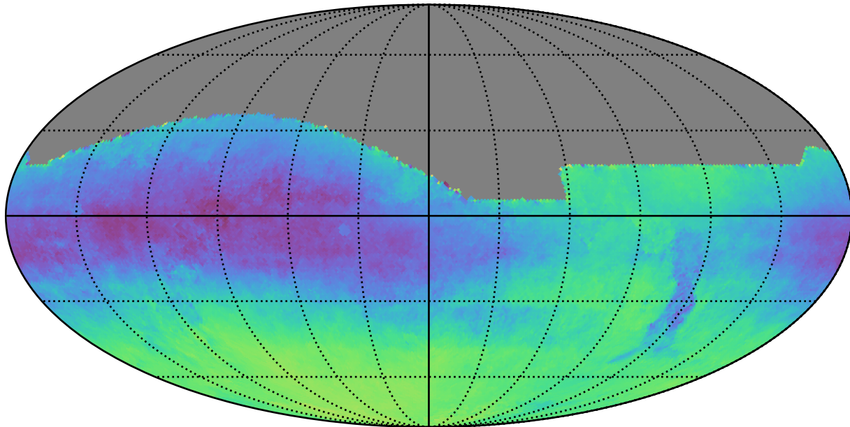
baseline_v3.2_10yrs All sky: Parallax-DCR degeneracy @ 24.0
