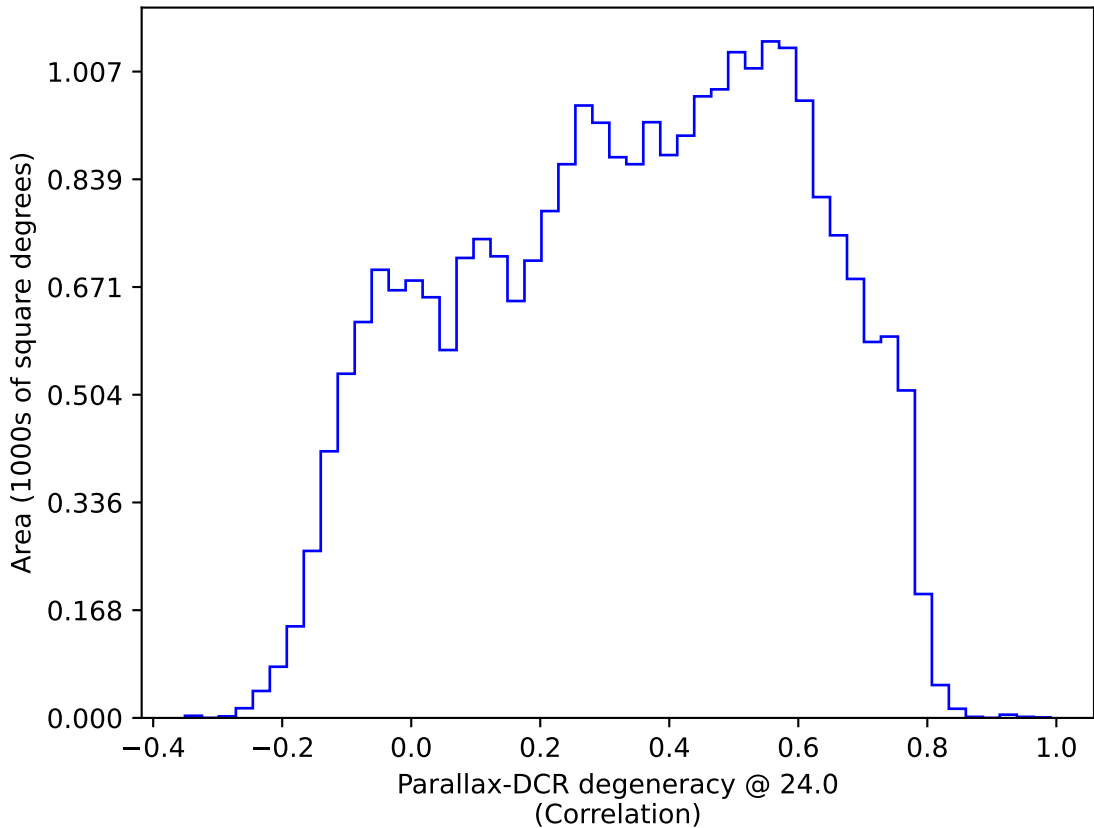
baseline_v3.2_10yrs All sky: Parallax-DCR degeneracy @ 24.0
