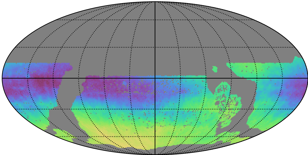
baseline_v3.2_10yrs WFD: Parallax-DCR degeneracy @ 22.4
