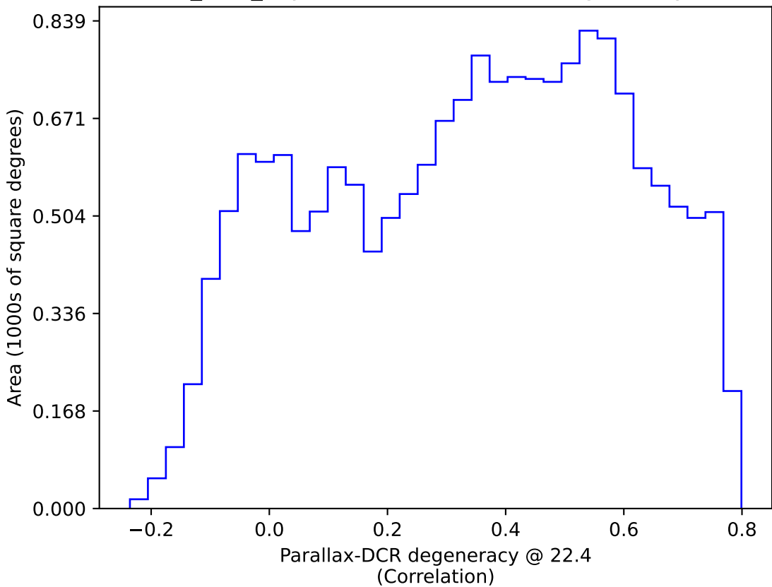
baseline_v3.2_10yrs WFD: Parallax-DCR degeneracy @ 22.4
