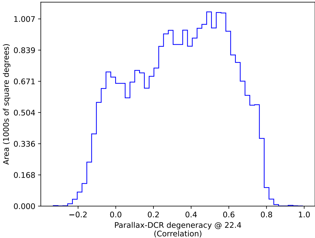
baseline_v3.2_10yrs All sky: Parallax-DCR degeneracy @ 22.4
