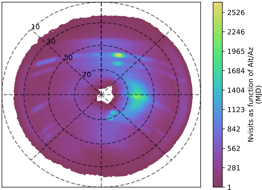
baseline_v3.2_10yrs z band: Nvisits as function of Alt/Az
