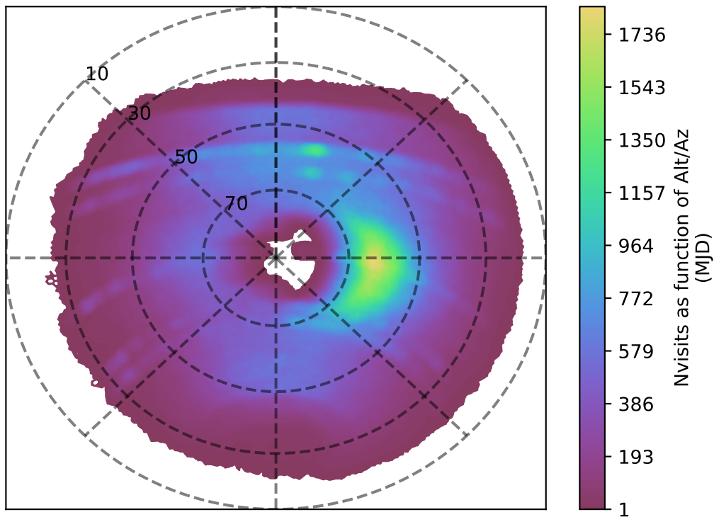
baseline_v3.2_10yrs y band: Nvisits as function of Alt/Az
