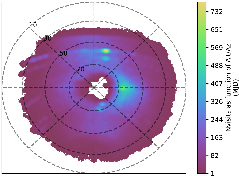
baseline_v3.2_10yrs u band: Nvisits as function of Alt/Az
