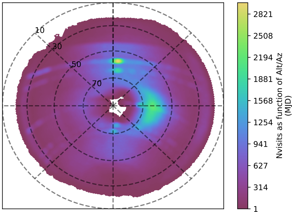
baseline_v3.2_10yrs i band: Nvisits as function of Alt/Az
