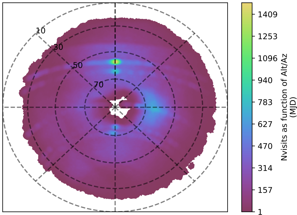
baseline_v3.2_10yrs g band: Nvisits as function of Alt/Az
