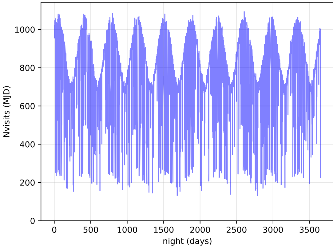
baseline_v3.2_10yrs All visits: Nvisits
