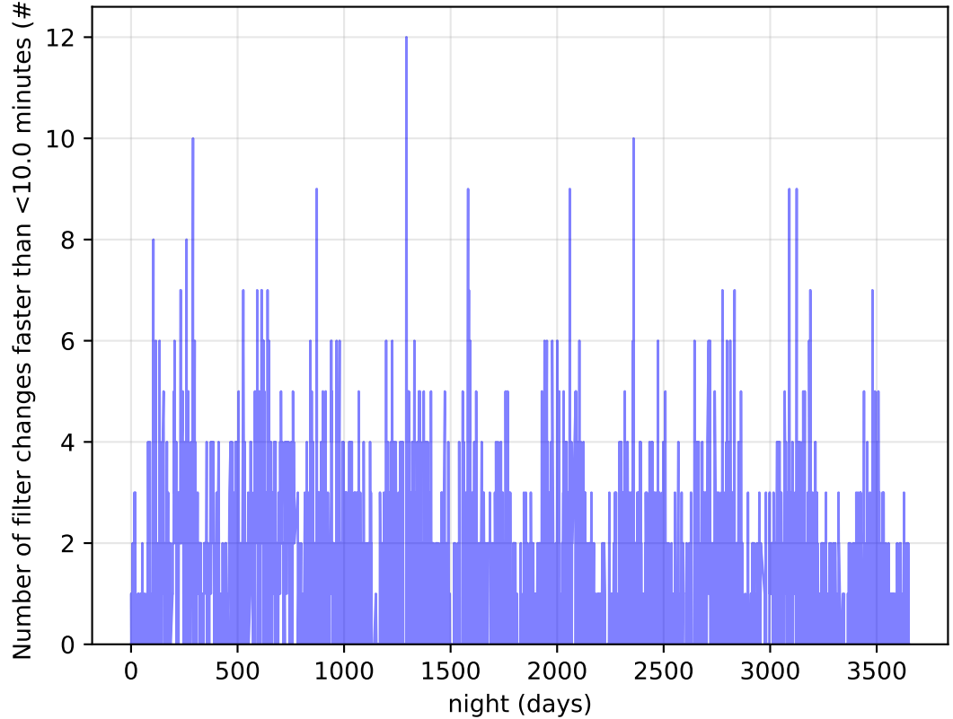
baseline_v3.2_10yrs Per Night: Number of filter changes faster than <10.0 minutes
