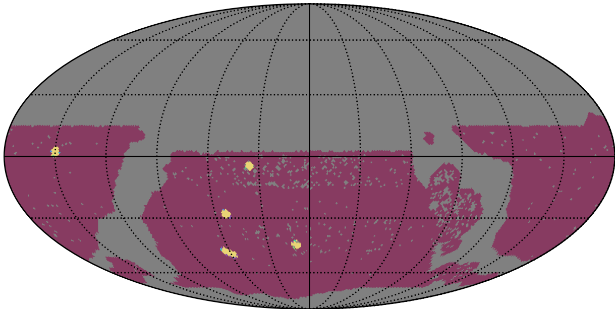
baseline_v3.2_10yrs WFD: NumberOfQuickRevisits
