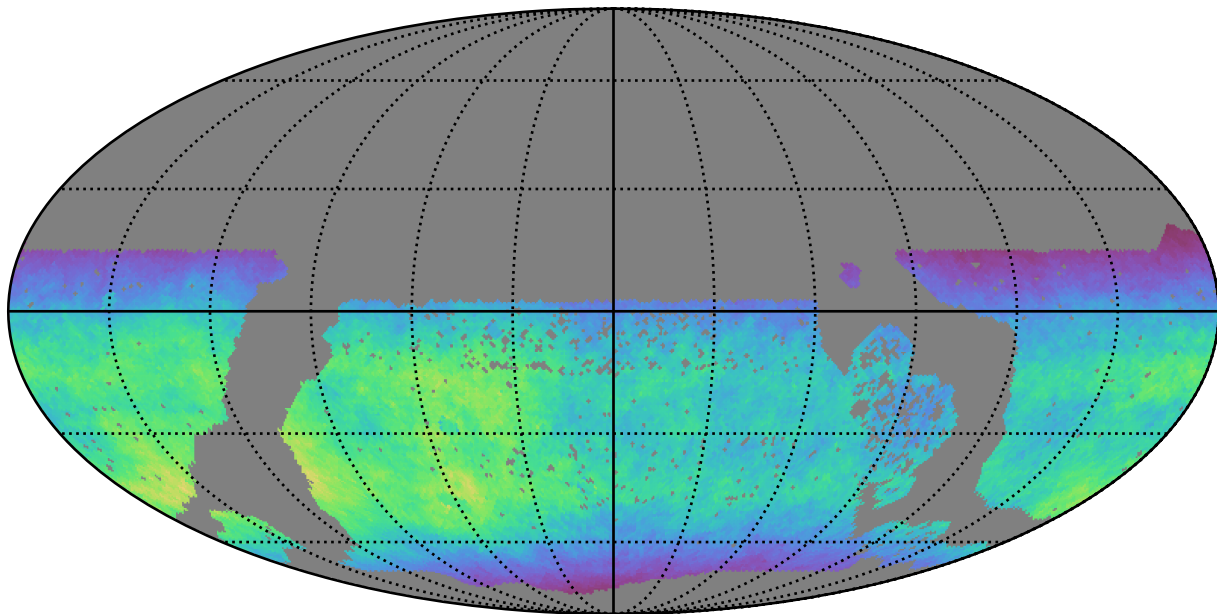
baseline_v3.2_10yrs WFD y band: Normalized Teff
