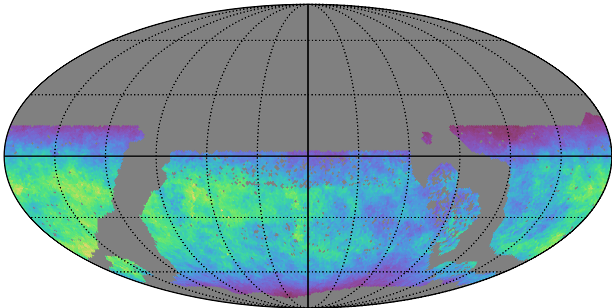
baseline_v3.2_10yrs WFD u band: Normalized Teff
