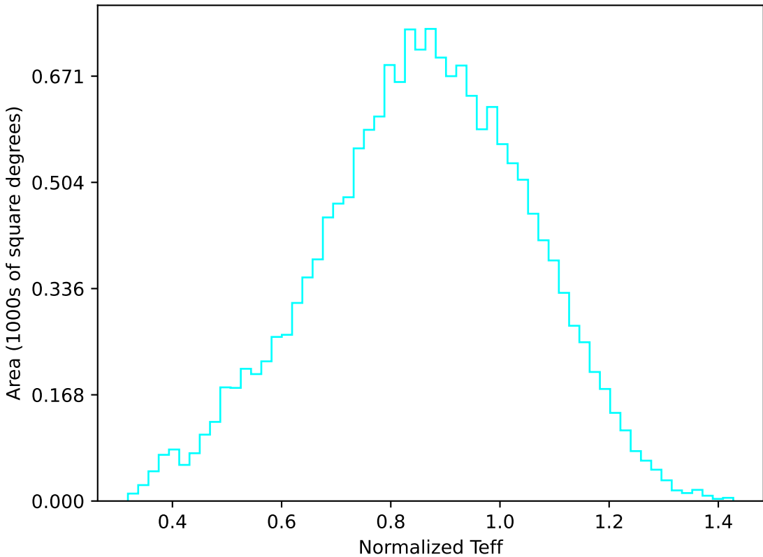
baseline_v3.2_10yrs WFD u band: Normalized Teff
