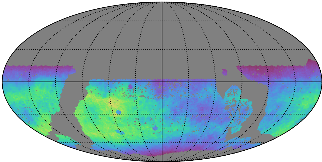
baseline_v3.2_10yrs WFD r band: Normalized Teff
