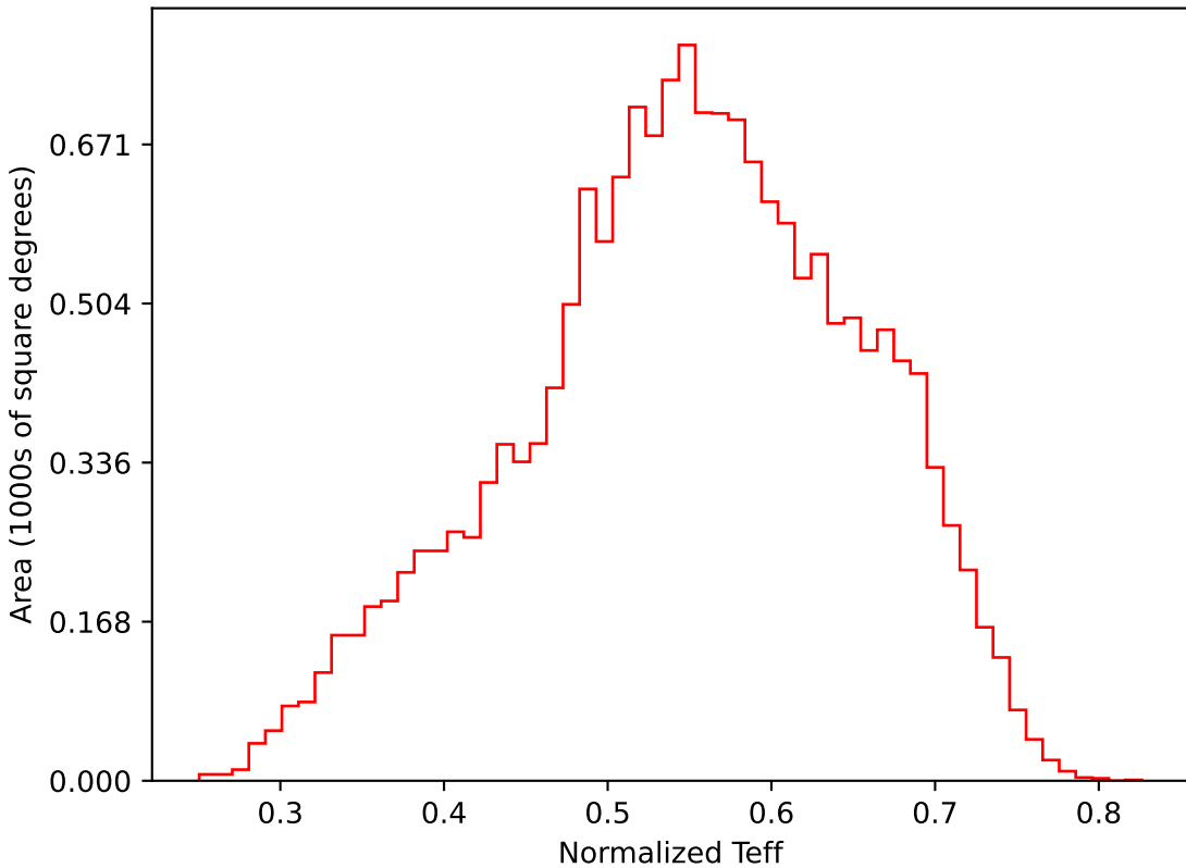
baseline_v3.2_10yrs WFD i band: Normalized Teff
