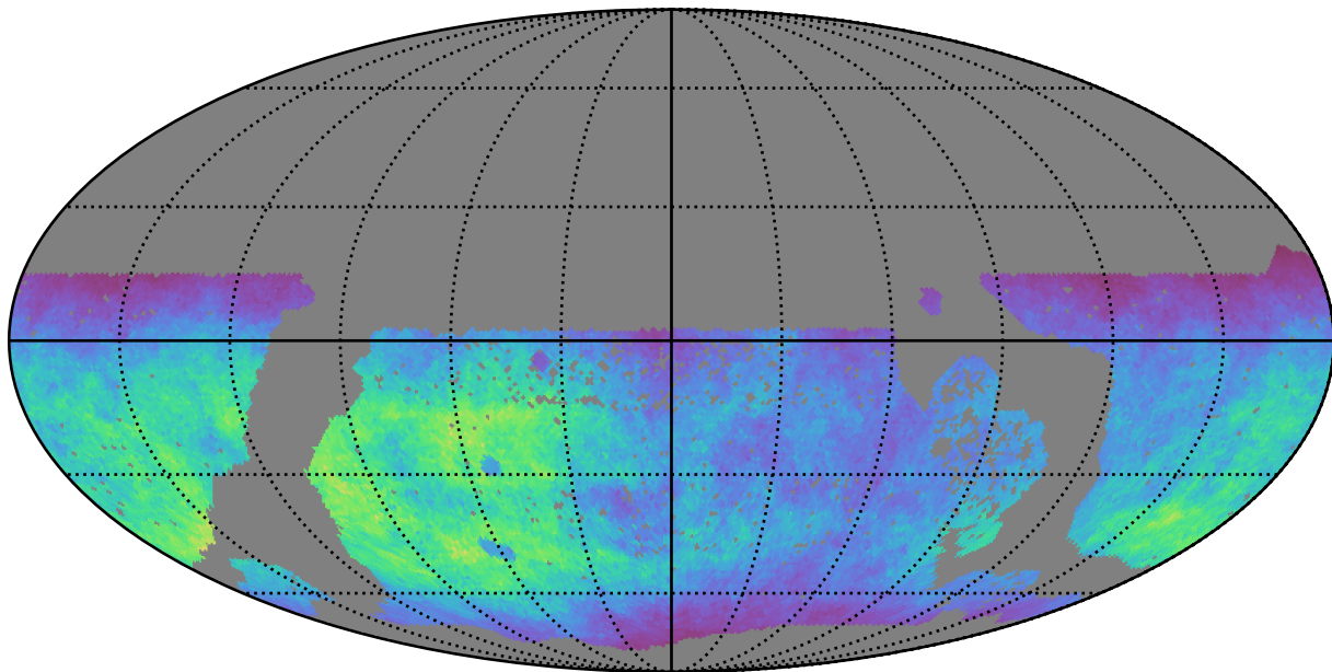
baseline_v3.2_10yrs WFD g band: Normalized Teff
