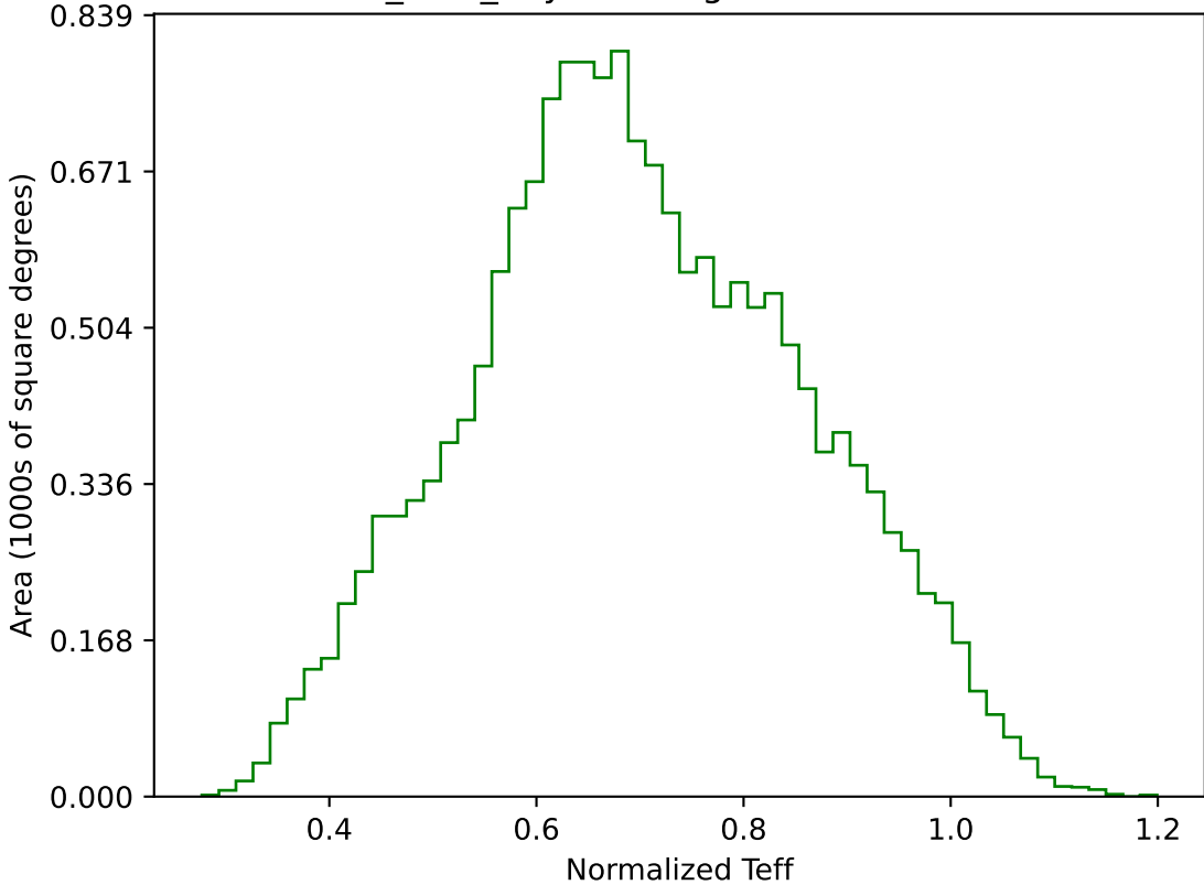
baseline_v3.2_10yrs WFD g band: Normalized Teff
