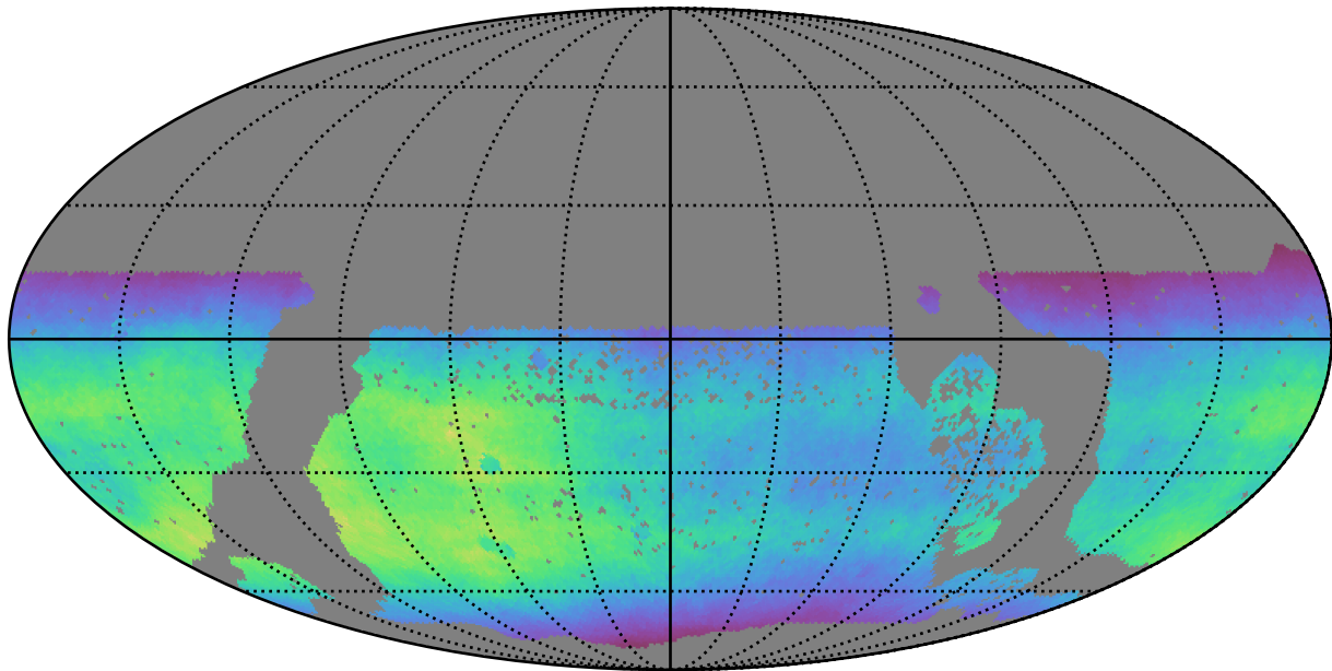
baseline_v3.2_10yrs WFD all bands: Normalized Teff
