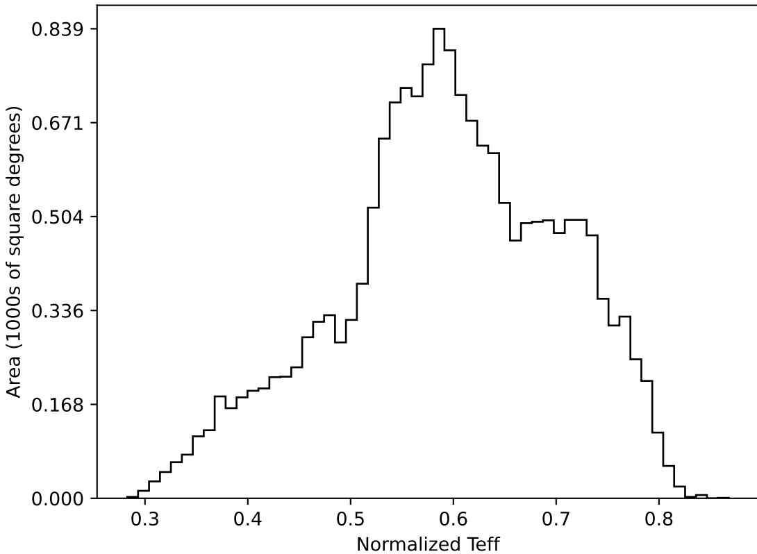
baseline_v3.2_10yrs WFD all bands: Normalized Teff
