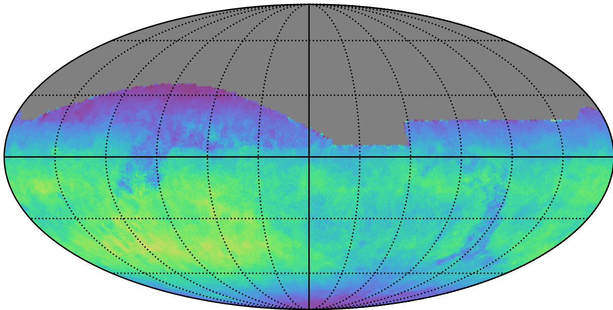
baseline_v3.2_10yrs All sky z band: Normalized Teff
