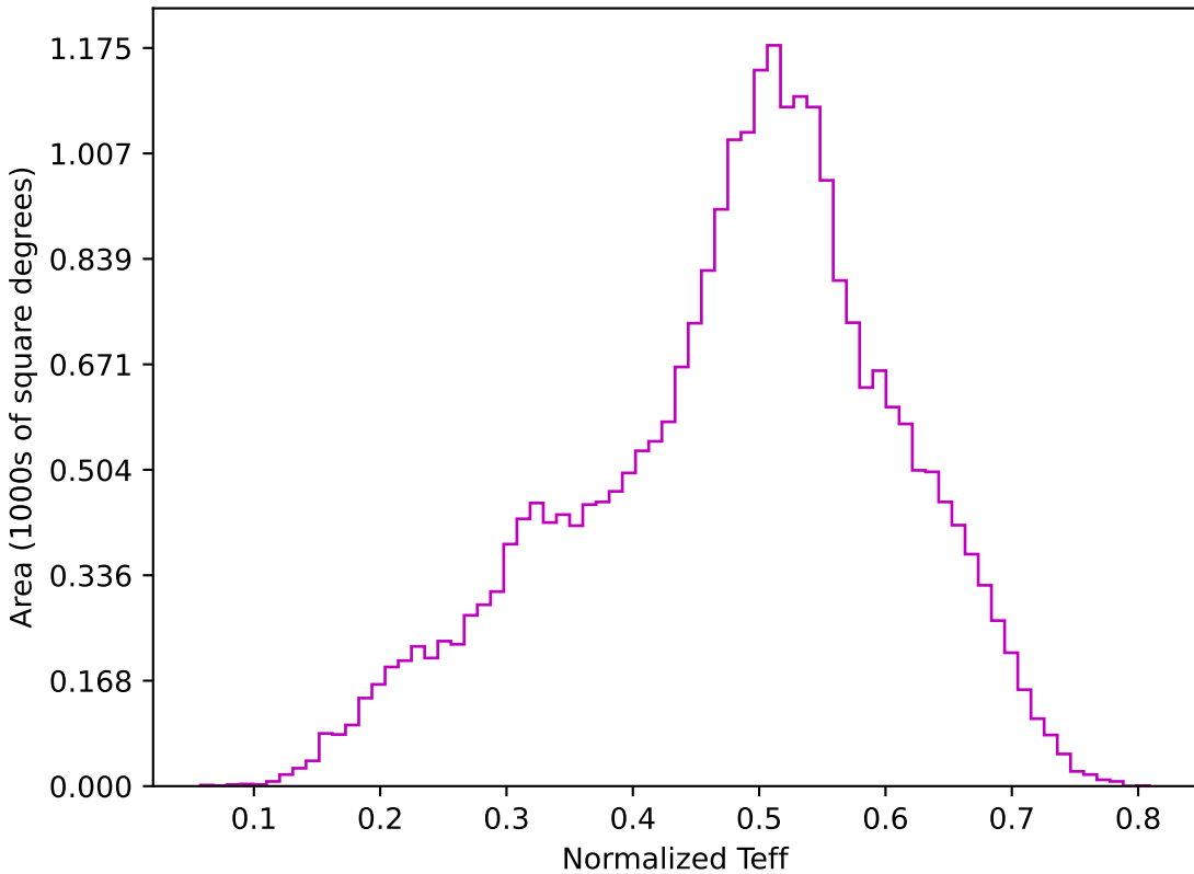
baseline_v3.2_10yrs All sky z band: Normalized Teff
