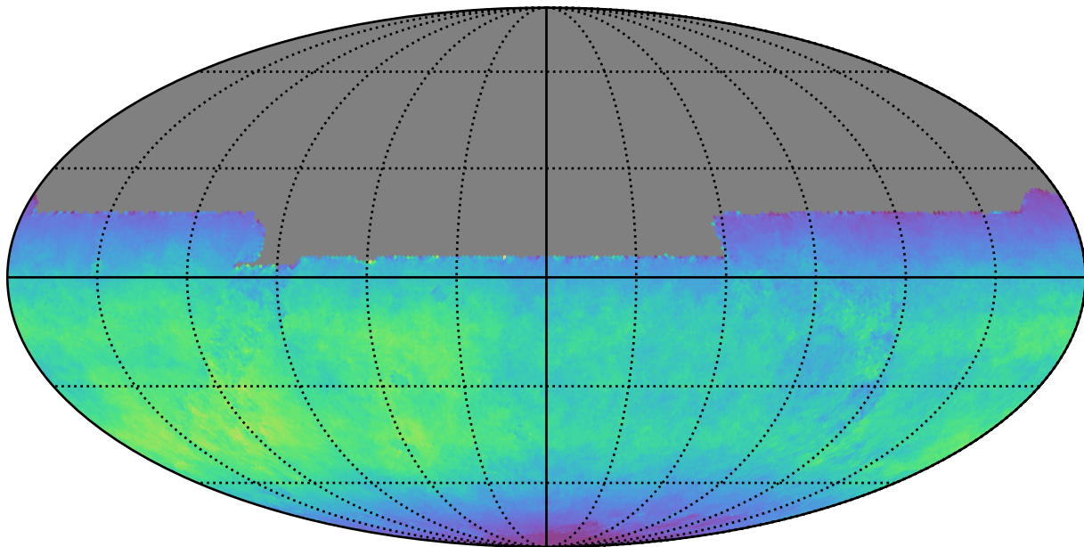
baseline_v3.2_10yrs All sky y band: Normalized Teff
