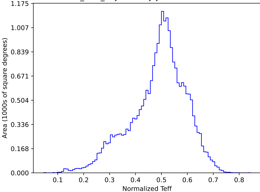
baseline_v3.2_10yrs All sky y band: Normalized Teff
