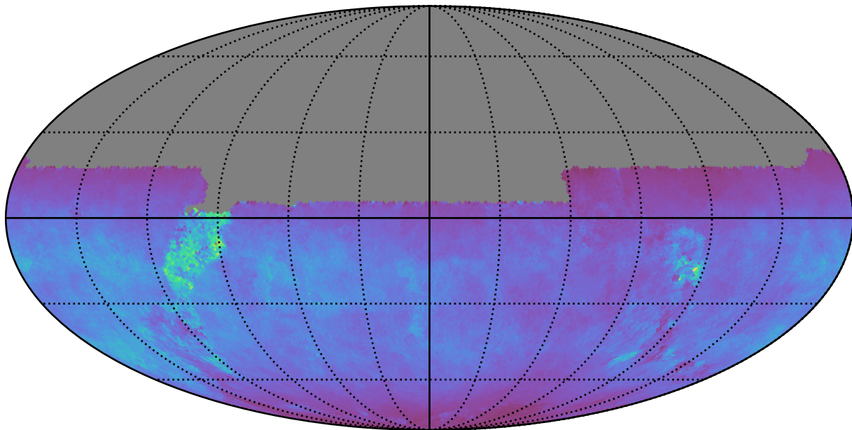
baseline_v3.2_10yrs All sky u band: Normalized Teff
