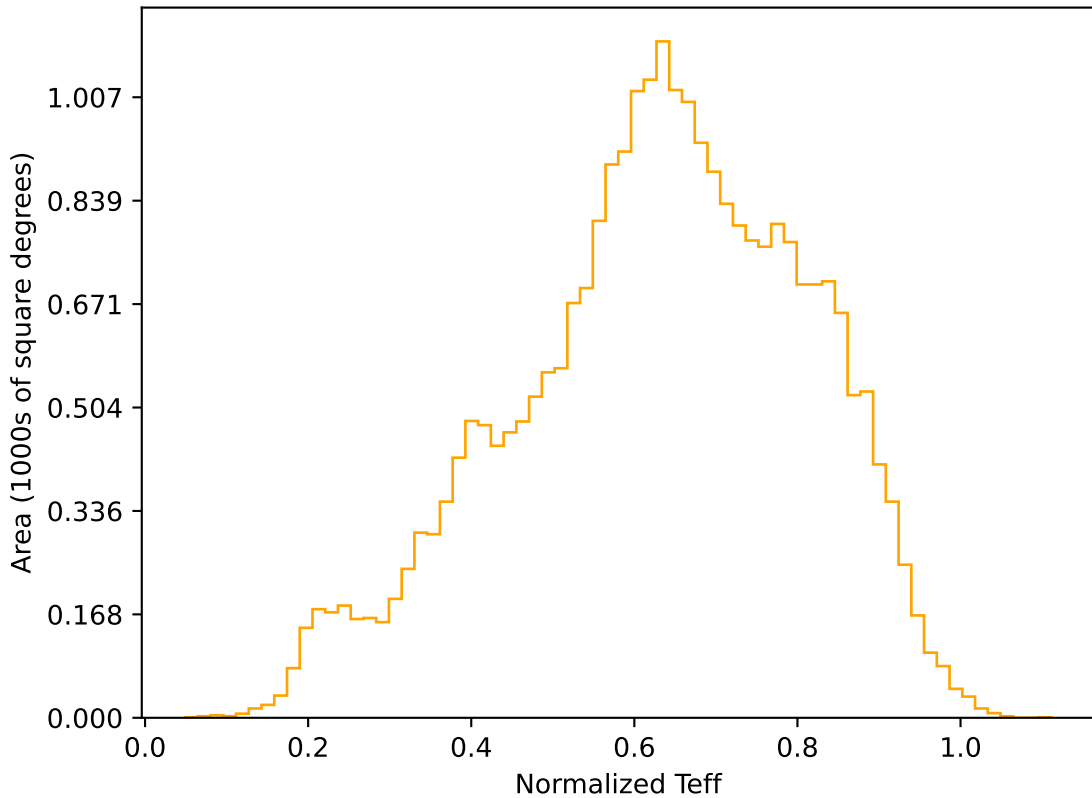
baseline_v3.2_10yrs All sky r band: Normalized Teff
