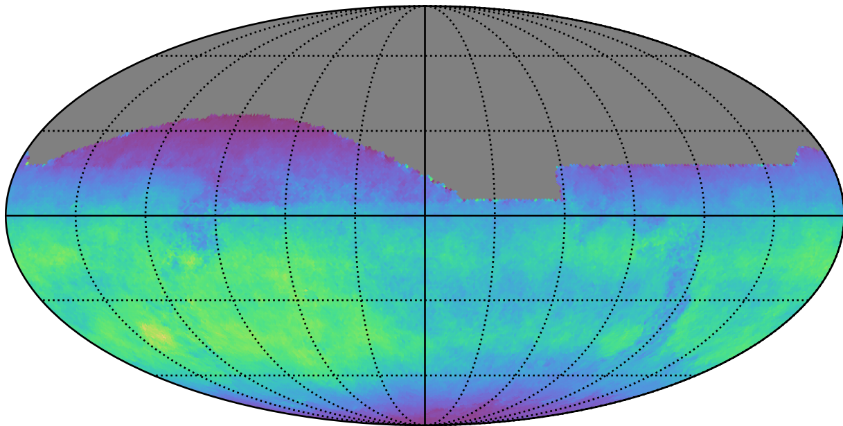
baseline_v3.2_10yrs All sky i band: Normalized Teff
