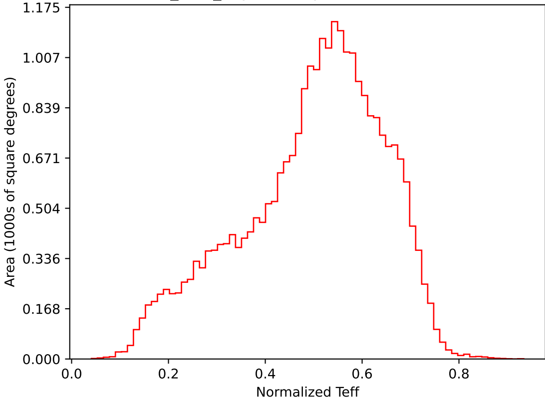
baseline_v3.2_10yrs All sky i band: Normalized Teff
